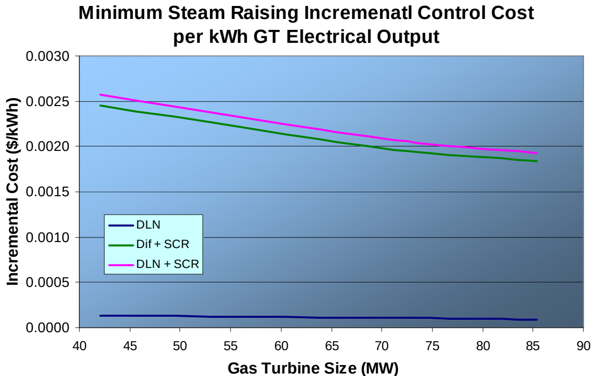
Figure B.6 - Minimum (330 kg/ GJ/h) Steam Raising, Control Costs for 1070°C Duct Firing
