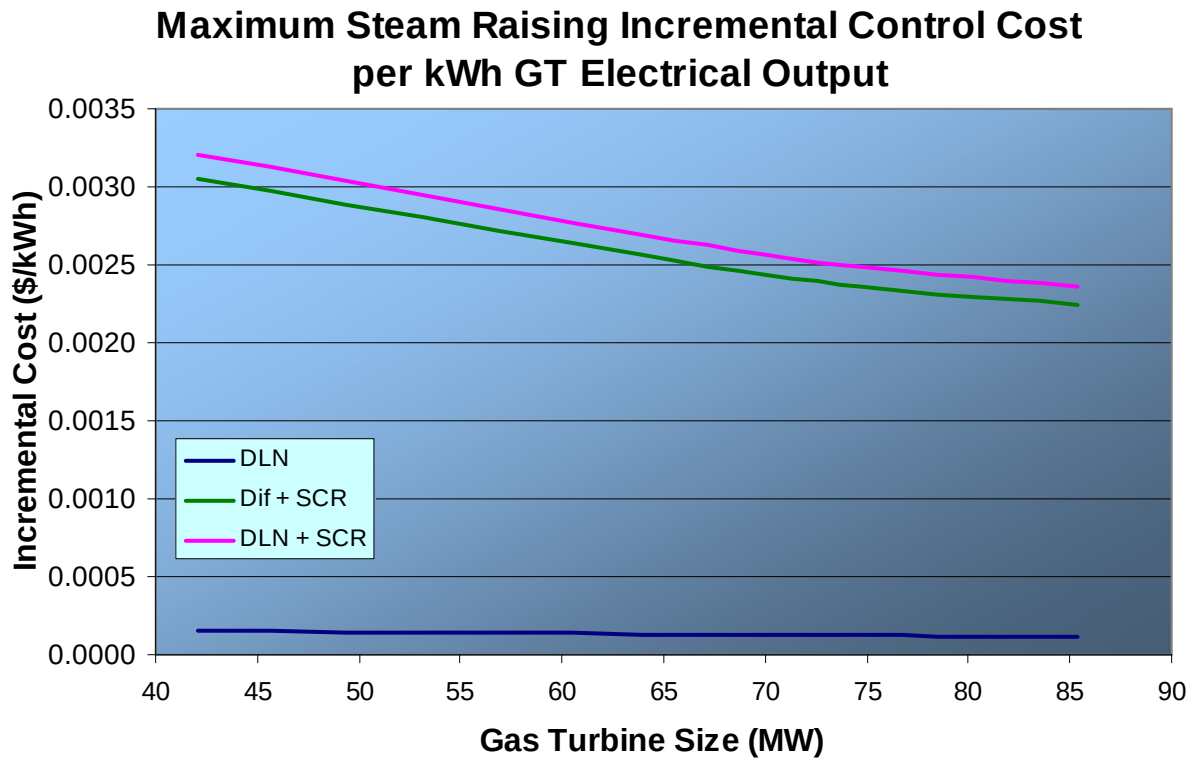
Figure B.9 - Maximum (440 kg/ GJ/h) Steam Raising, Control Costs for 840°C Duct Firing
