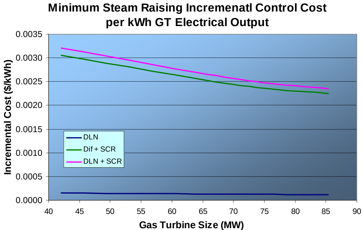
Figure B.10 - Minimum (330 kg/ GJ/h) Steam Raising, Control Costs for 840°C Duct Firing
