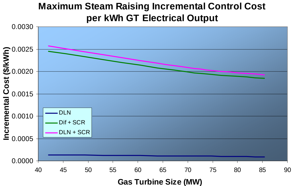
Figure B.5 - Maximum (440 kg/ GJ/h) Steam Raising, Control Costs for 1070°C Duct Firing
