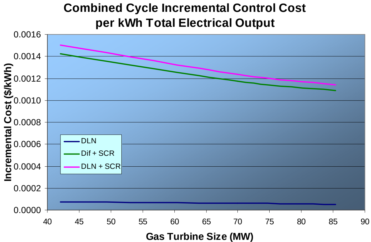
Figure B.3 - Combined Cycle Control Costs for 1070°C Duct Firing
