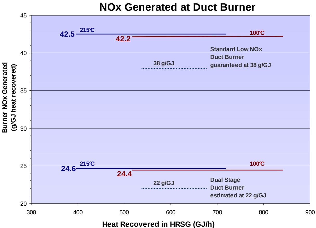
Figure D.3 - Burner NOx (per unit heat recovered) Varying with Heat Recovered
